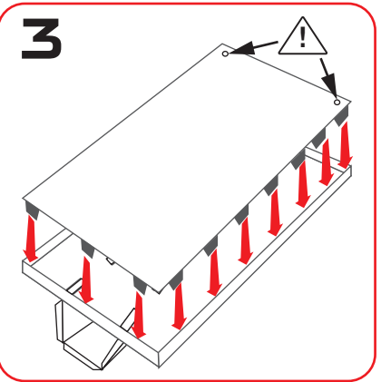
ASSEMBLE PART 1 + PART 3 ⚠ Use the holes to hang the stand to a wall if needed.
